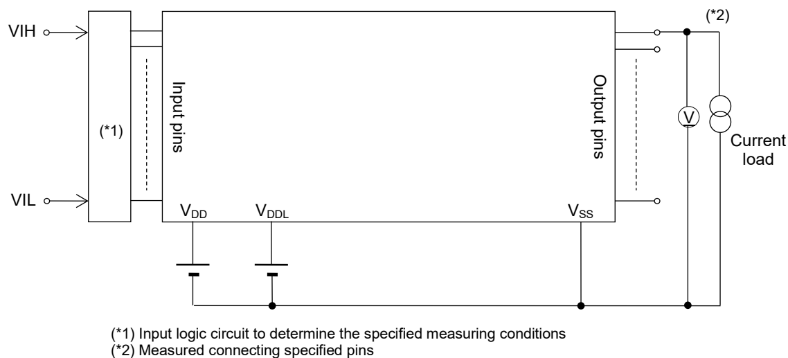
Measuring circuit 3
