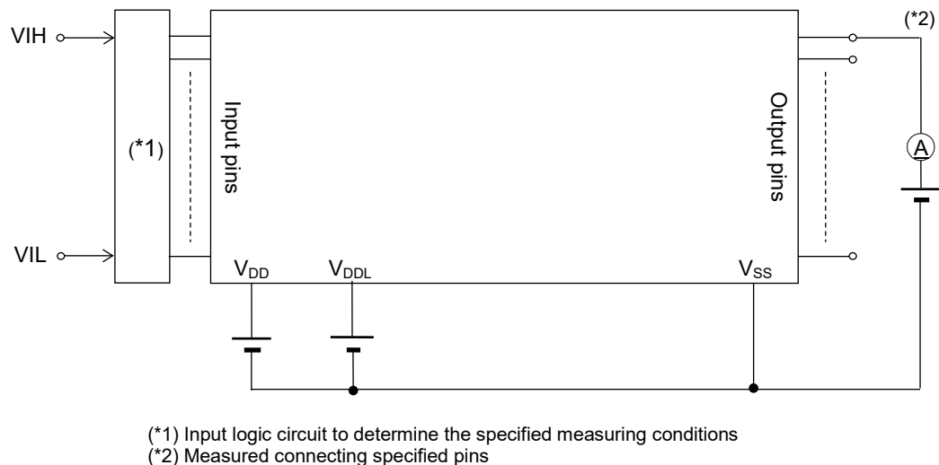
Measuring circuit 3
