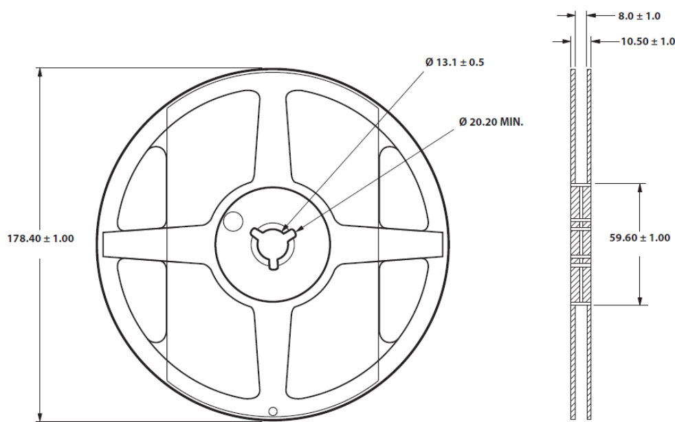
Figure 8: Reel Dimensions
