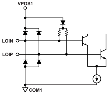
Figure 3. Circuit A
