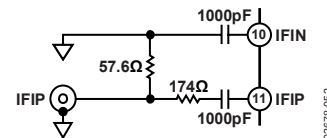
Figure 52. Minimum-Loss L Pad for 50 \Omega IF Input
