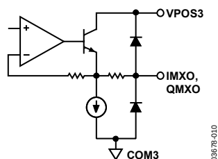
Figure 10. Circuit H
