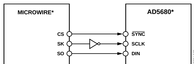
Figure 31. AD5680 to MICROWIRE Interface
