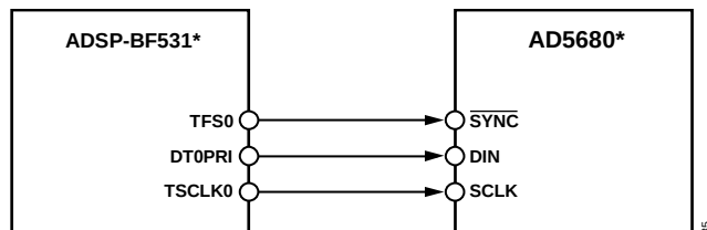
Figure 28. AD5680 to Blackfin ADSP-BF531 Interface
