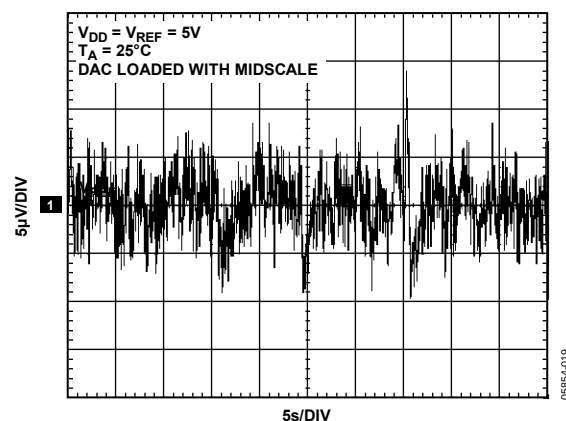
Figure 21. 0.1 Hz to 10 Hz Output Noise Plot
