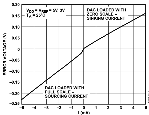
Figure 10. Headroom at Rails vs. Source and Sink Current
