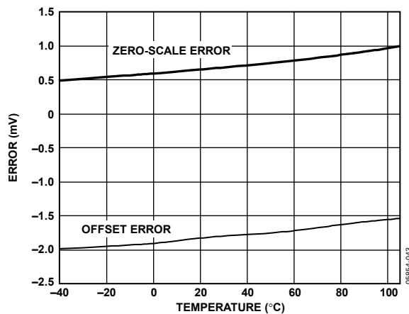
Figure 9. Zero-Scale Error and Offset Error vs. Temperature
