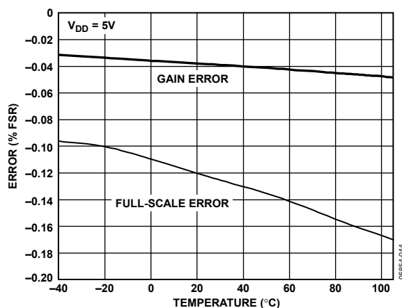
Figure 8. Gain Error and Full-Scale Error vs. Temperature
