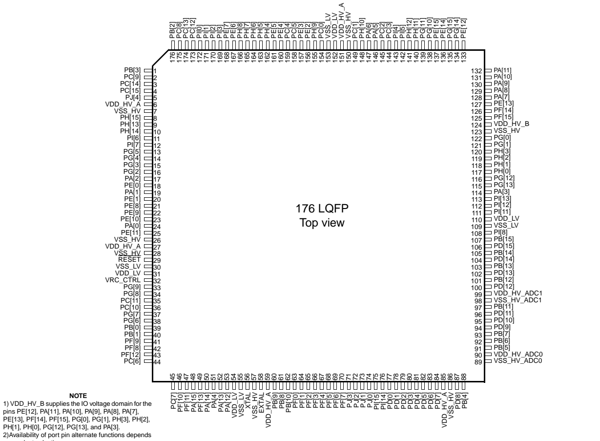
Figure 2. 176-pin LQFP configuration
