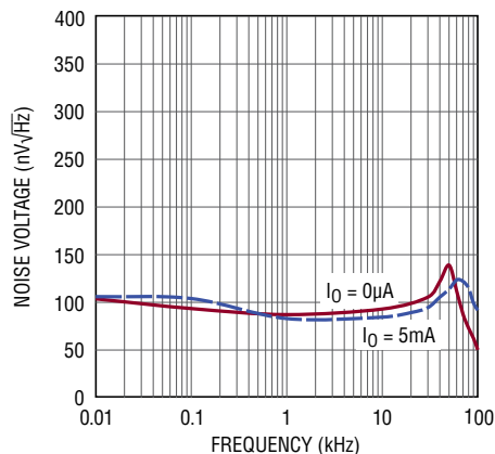
1.2V Output Voltage Noise Spectrum
