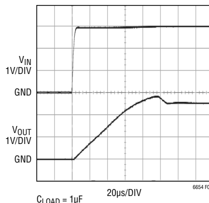
Figure 1. Turn-On Characteristics of LT6654-2.5
