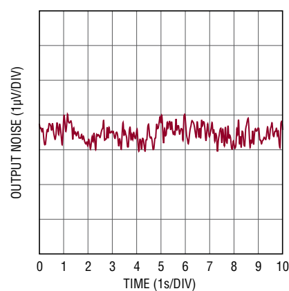
1.25V Output Noise 0.1Hz to 10Hz
