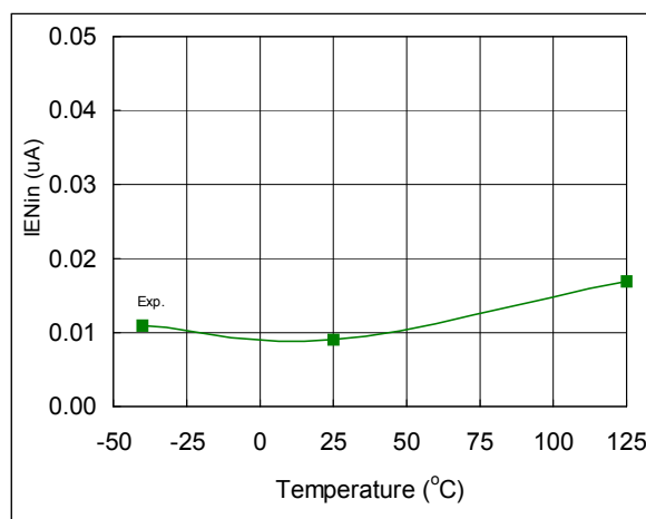
Fig. 117. En Input Bias Current vs. Temperature
