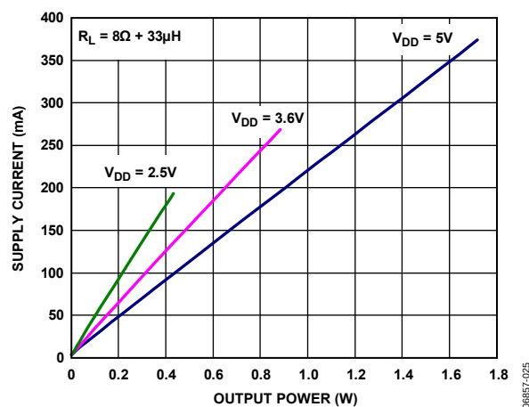
Figure 25. Supply Current vs. Output Power, R_L = 8\Omega + 33\mu\text{H}
