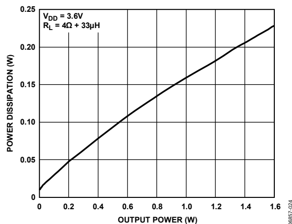
Figure 24. Power Dissipation vs. Output Power, R_L = 4\Omega + 33\mu\text{H} at V_{DD} = 3.6\text{V}
