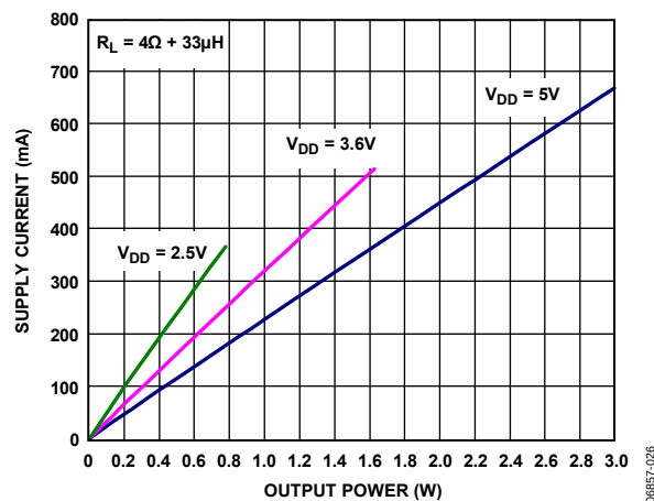
Figure 26. Supply Current vs. Output Power, R_L = 4\Omega + 33\mu\text{H}
