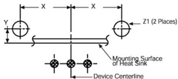
Mounting Details:
