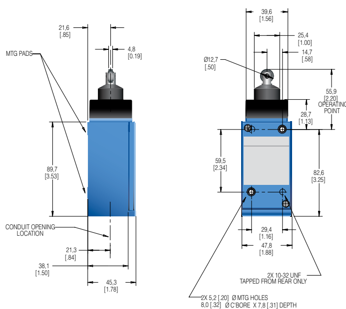
DPDT Non-plug-in (mm[in])
