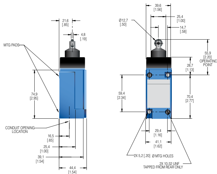
SPDT Plug-in (mm[in])
