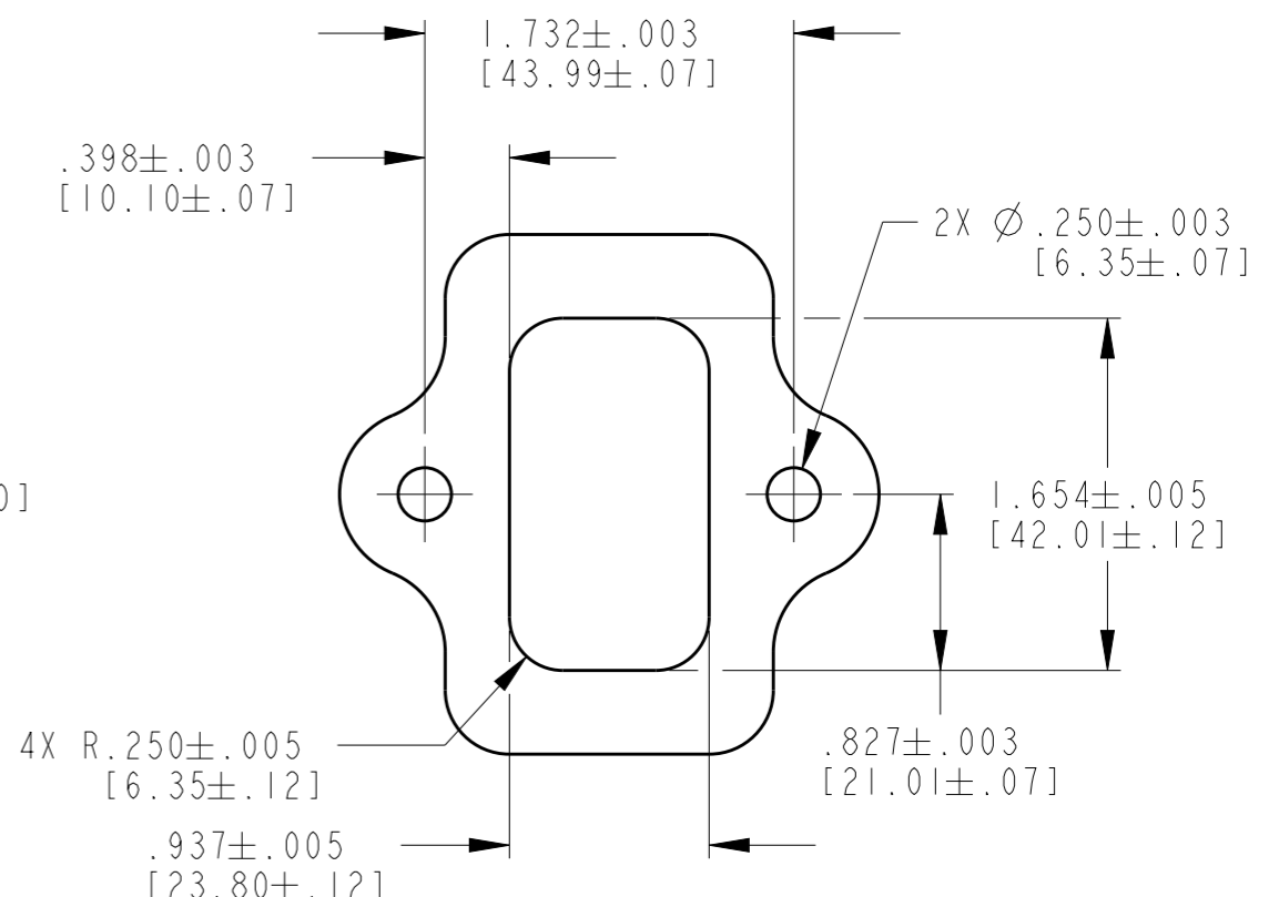
RECOMMENDED MOUNTING DETAIL
