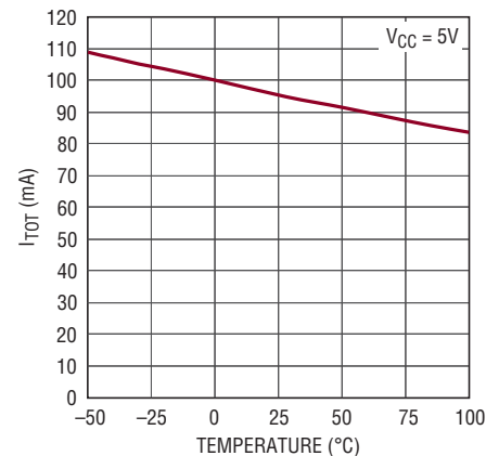
Total Current ( I_{\text{TOT}} ) vs Temperature
