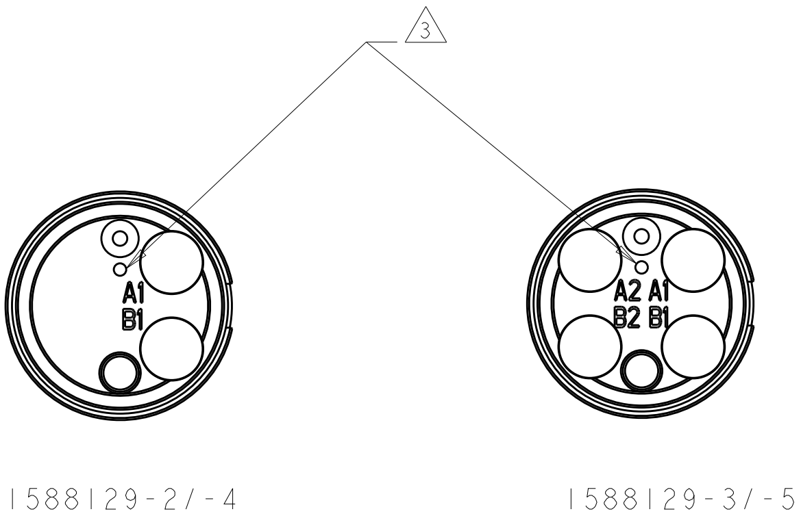
VIEW X - X (SHOWN WITHOUT PROTECTIVE LABEL)
