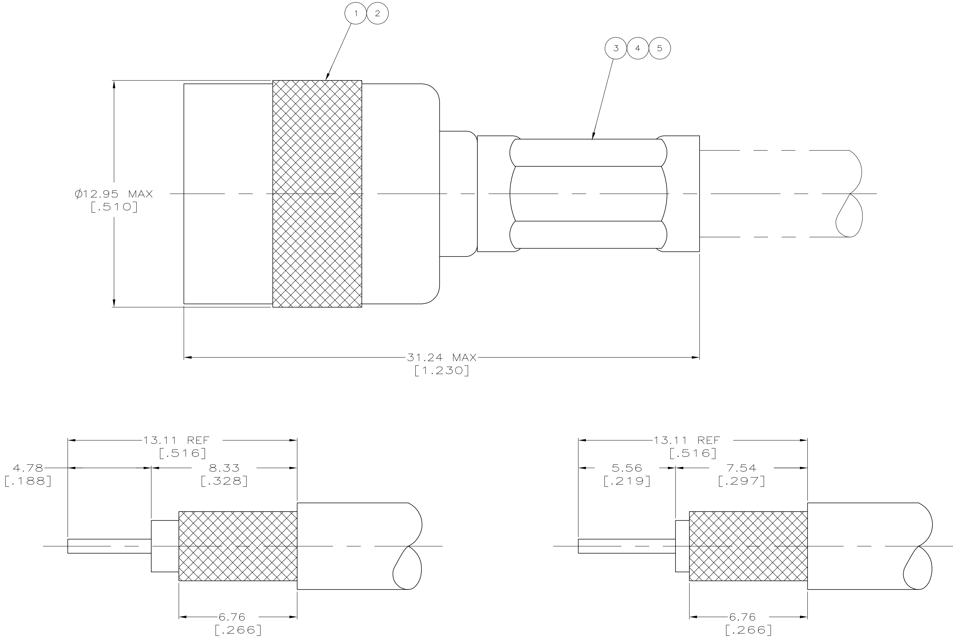
RECOMMENDED STRIP LENGTH
