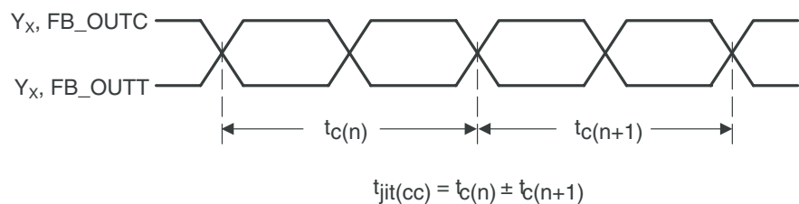
Figure 3. Cycle-to-Cycle Jitter
