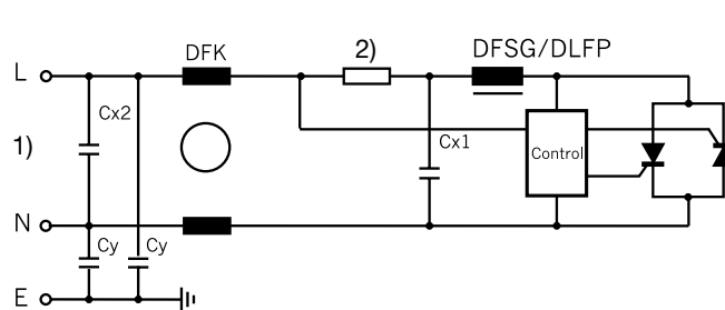
Interference suppression with resistive load, 2-stage
