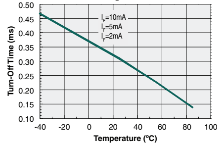
Typical Turn-Off Time vs. Temperature ( V_L=10V )
