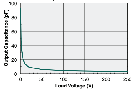
Typical Output Capacitance vs. Load Voltage ( I_F=0mA , f=1MHz )
