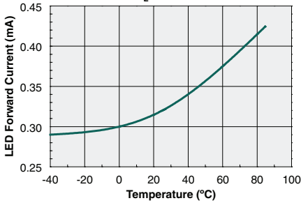
Typical I_F to Operate vs. Temperature ( I_L=100mA )
