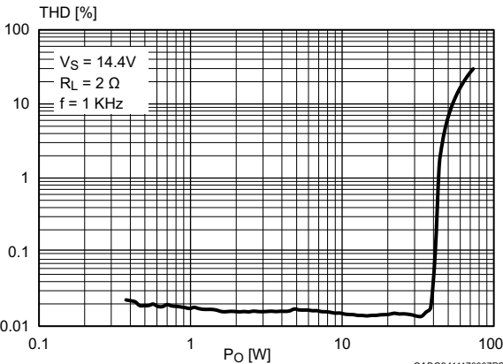
Figure 26. THD vs. output power ( V_S = 14.4\text{ V} , R_L = 2\ \Omega )
