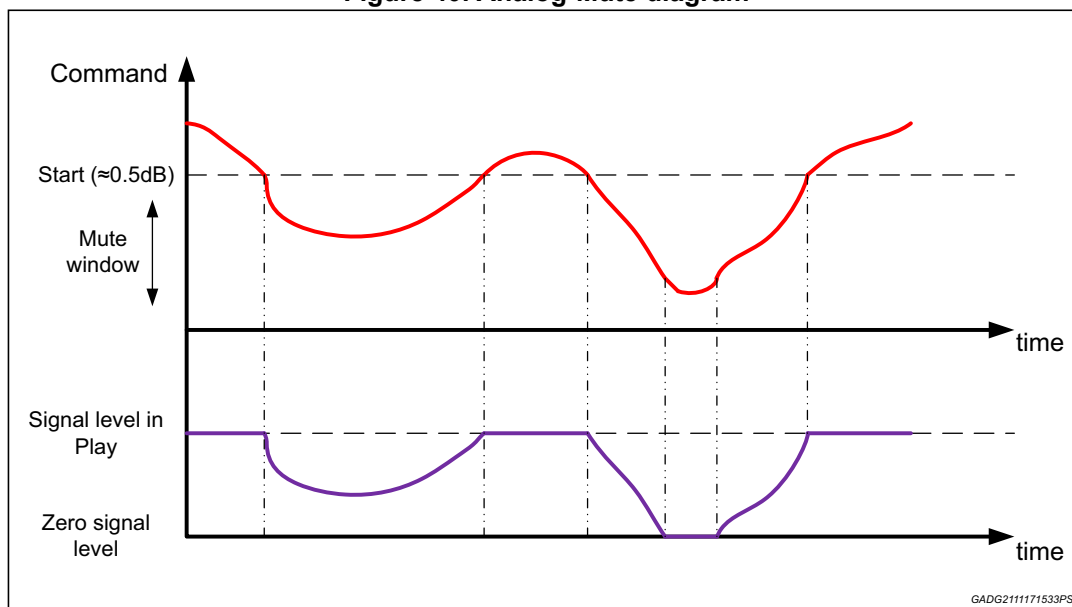
Figure 40. Analog-Mute diagram
