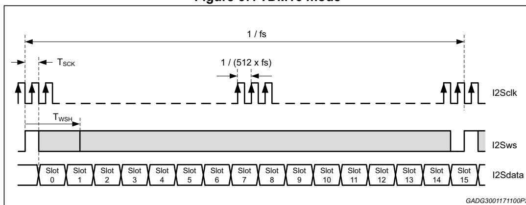
Figure 67. TDM16 mode
