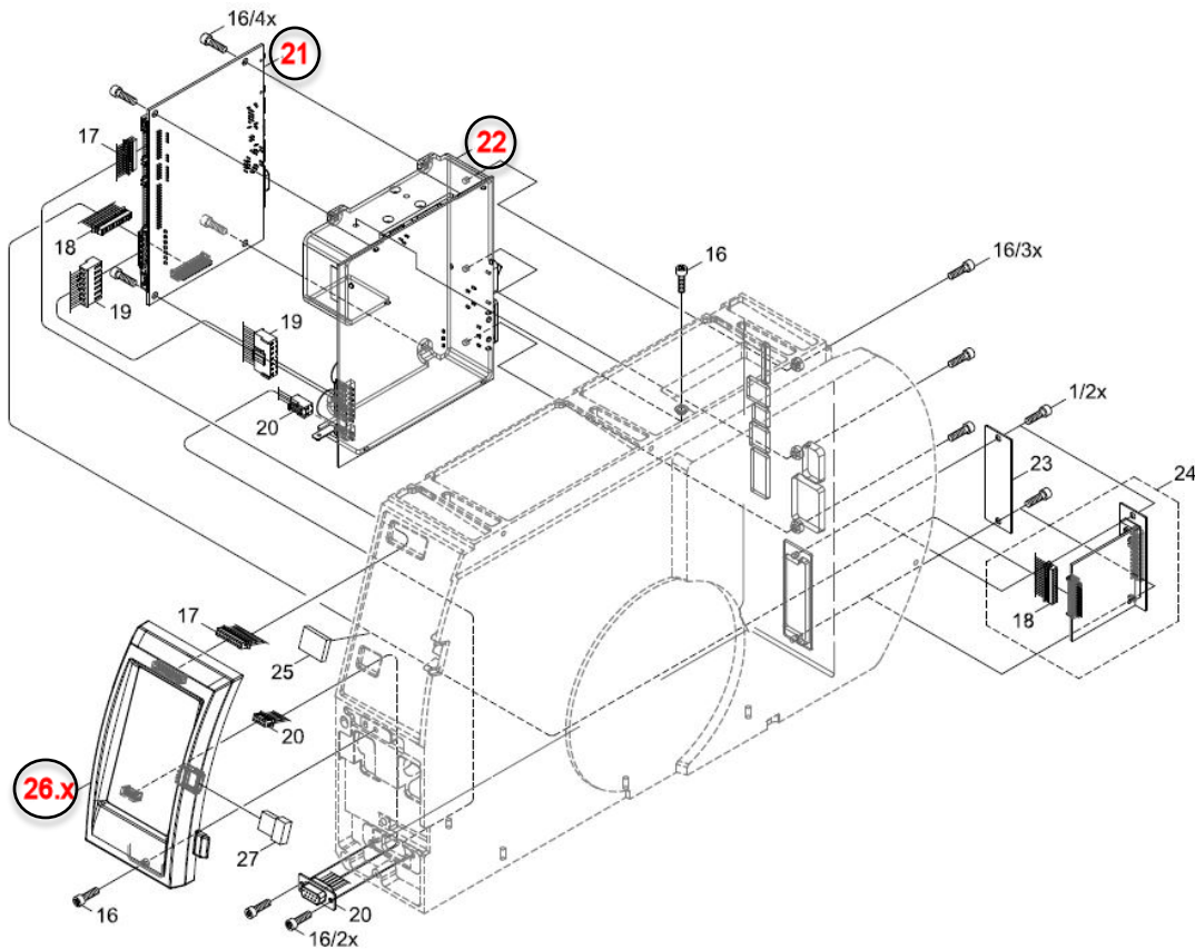
Figure 4 - T3212/T3224-PRINTER (electronics)
