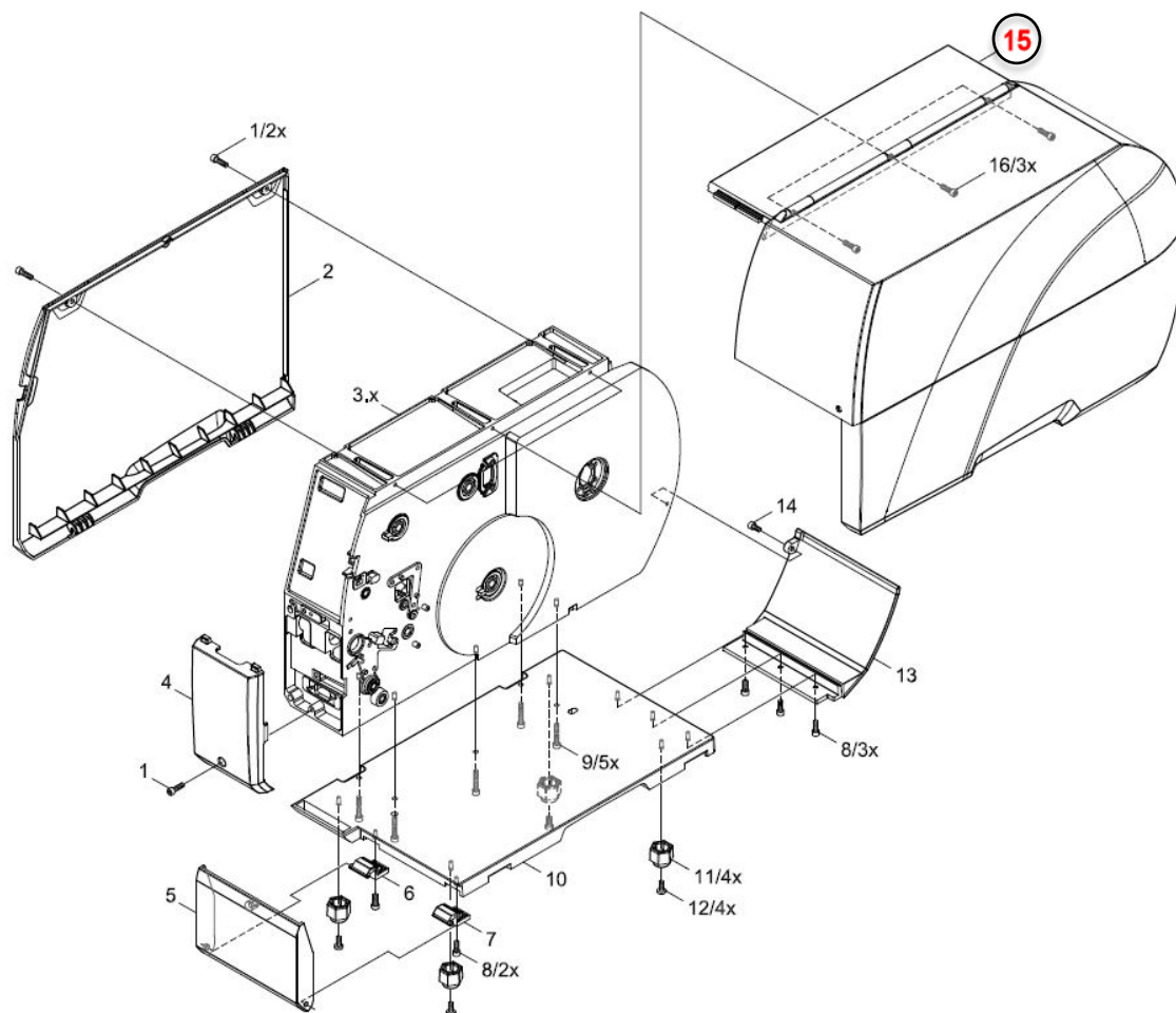
Figure 3 - T3212/T3224-PRINTER (cover)
