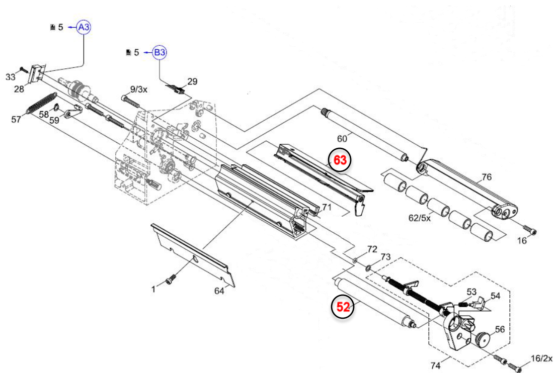
Figure 6 - T3212/T3224-PRINTER (drive rollers/Sensor)
