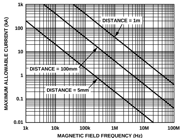
Figure 34. Maximum Allowable Current for Various Current to ADuM4137 Spacings
