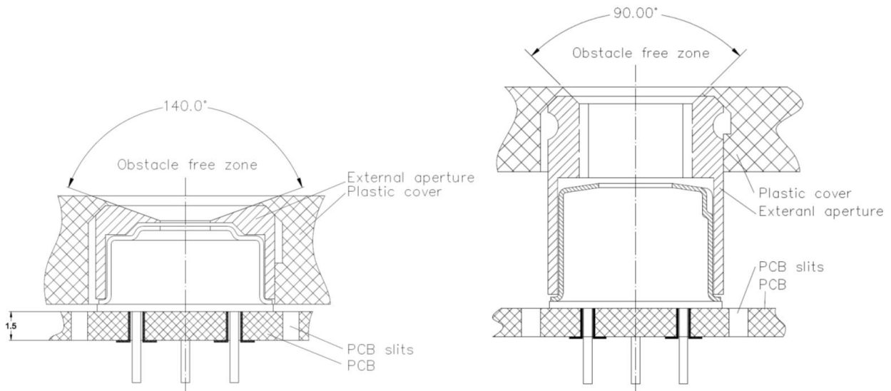
Figure 25 Application examples concerning the optical consideration
