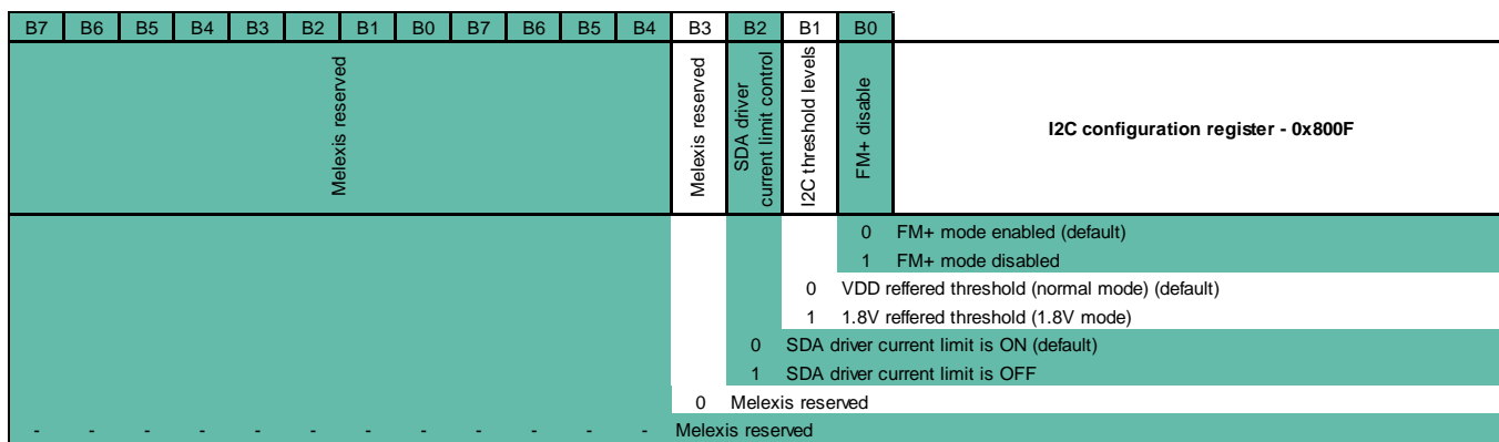
Figure 13 I 2 C configuration register (0x800F) bits meaning
