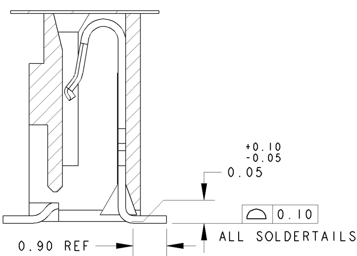
SECTION B-B (FOR ODD POSITION CONTACTS) SCALE 10:1
