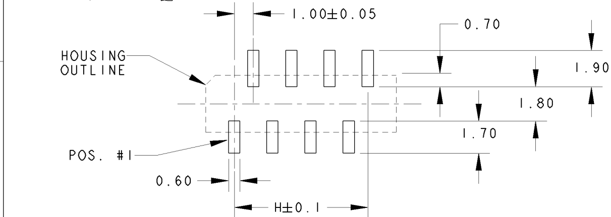
RECOMMENDED PCB LAYOUT (NON-ACCUMULATIVE TOLERANCE) (FOR EVEN POSITION CONNECTORS)
