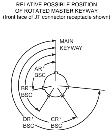
RELATIVE POSSIBLE POSITION OF ROTATED MASTER KEYWAY (front face of Tri-Start connector receptacle shown)
