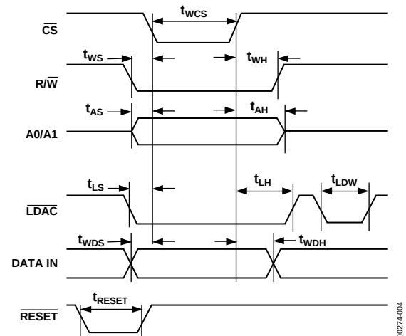
Figure 4. Data Write (Input and Output Registers) Timing
