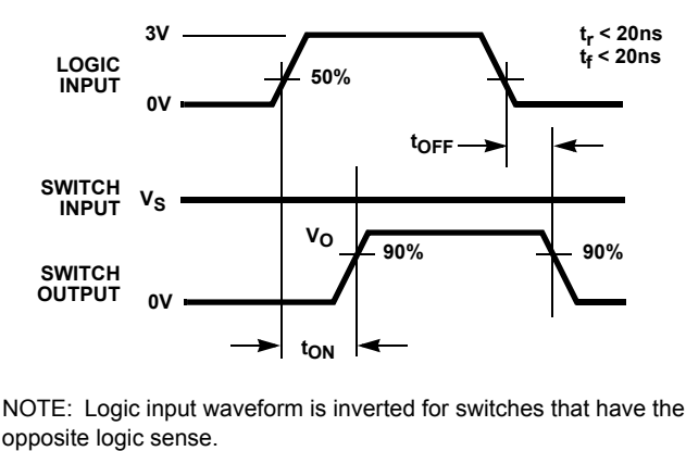
FIGURE 1A. MEASUREMENTS POINTS
