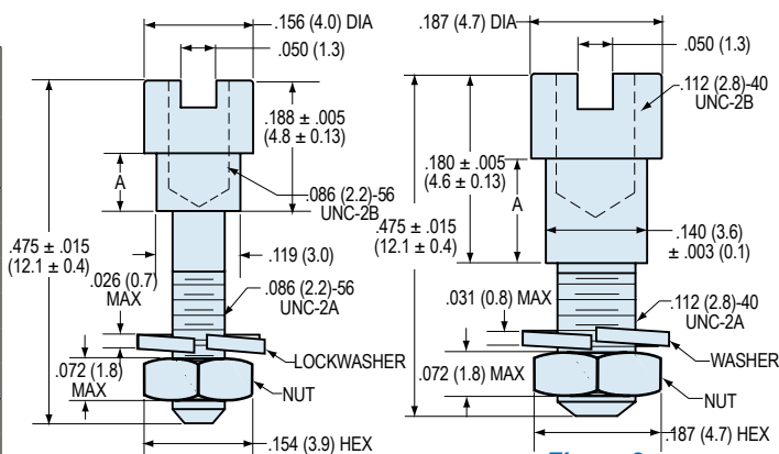
Figure 1 #2-56 Jackpost
