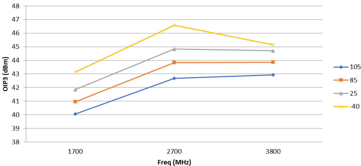
GRF4014 Evaluation Board OIP3 vs. Frequency vs. Temperature; Vdd: 8.0 Volts
