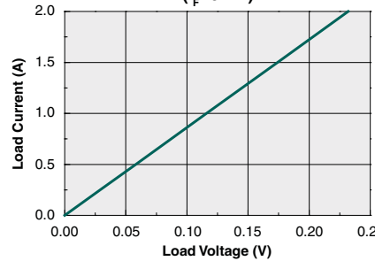
Load Current vs. Load Voltage DC-Only Configuration ( I_F=0\text{mA} )
