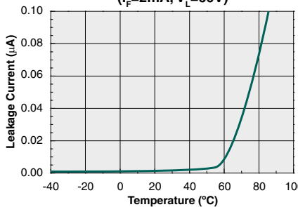
Typical Leakage Current vs. Temperature ( I_F=2\text{mA} , V_L=60\text{V} )
