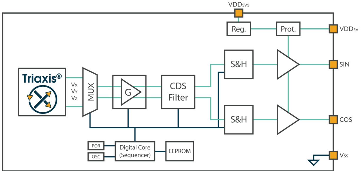
Figure 3: Functional Diagram
