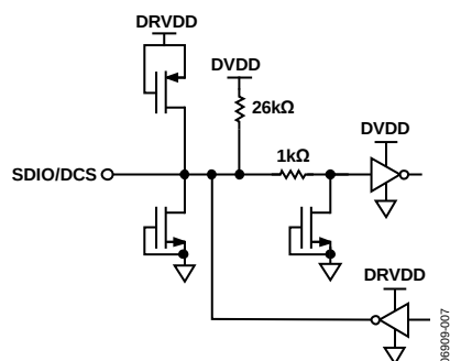
Figure 11. Equivalent SDIO/DCS Input Circuit
