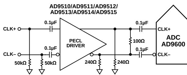
Figure 58. Differential PECL Sample Clock (up to 150 MSPS)
