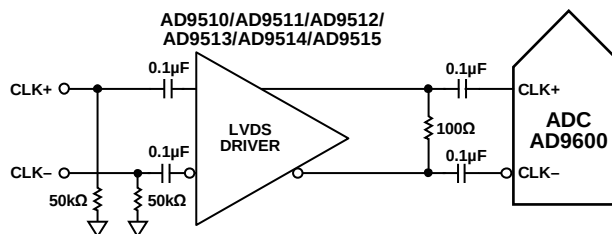
Figure 59. Differential LVDS Sample Clock (up to 150 MSPS)
