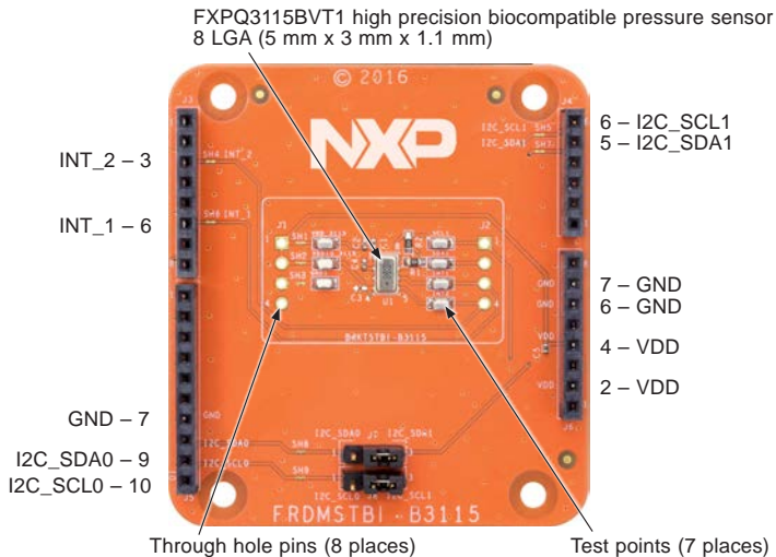
Figure 1: FRDMSTBI-B3115
