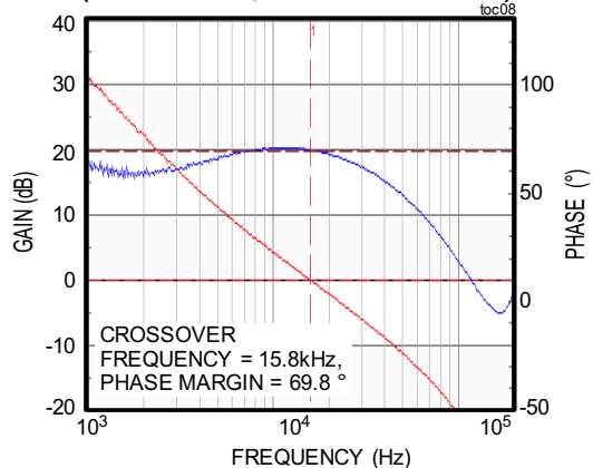
BODE PLOT (3.3V OUTPUT, 1A LOAD CURRENT)
