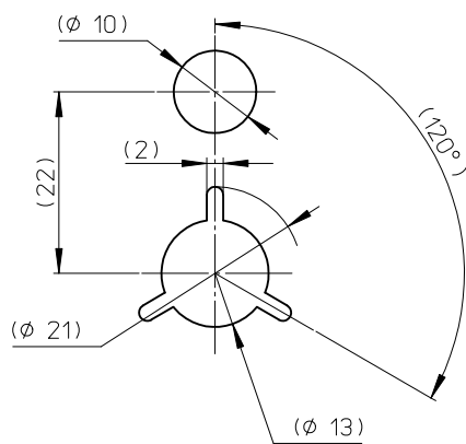
DETAIL "E"
