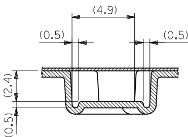
SECT.X-X
