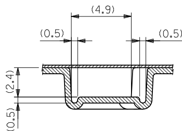
SECT. W-W
