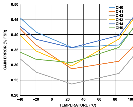
Figure 32. Gain Error vs. Temperature
