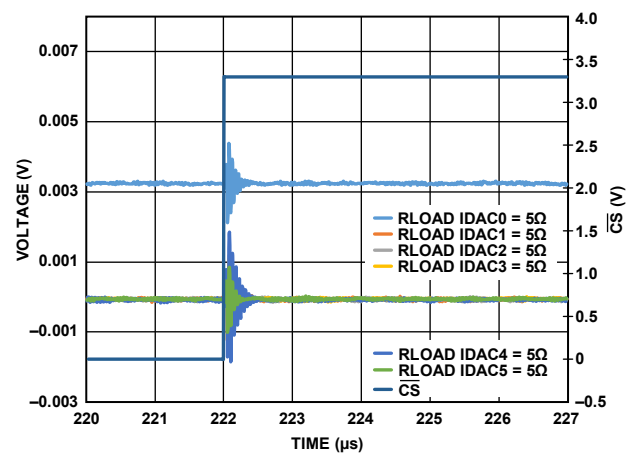
Figure 56. Analog Crosstalk
