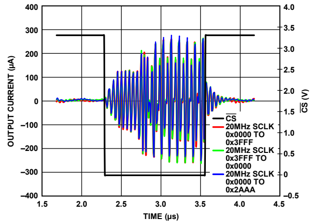
Figure 54. Digital Feedthrough
