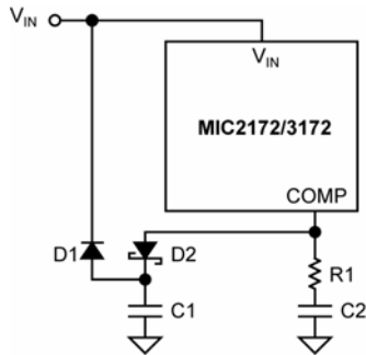
Figure 8. Soft Start
