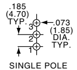
SINGLE POLE
