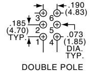
DOUBLE POLE
