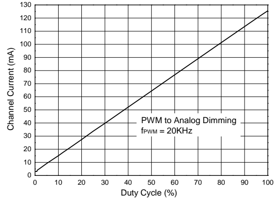
PWM to Analog Dimming @ f PWM = 20kHz Channel Current vs. Duty Cycle
