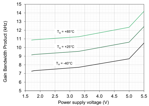
Fig 16. Gain Bandwidth Product vs. Power Supply Voltage
