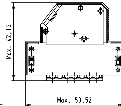
Hood upper part
