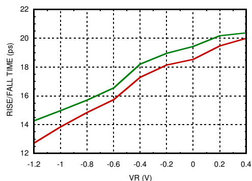
Rise / Fall Time vs. VR [2][3]
