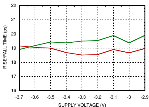
Rise / Fall Time vs. Supply Voltage [1][2]
