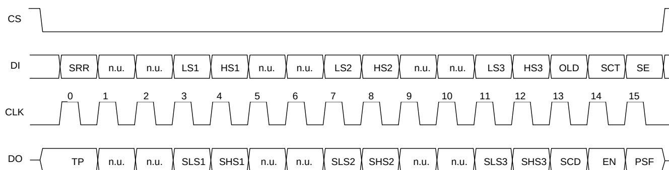
Figure 2: Data Transfer
