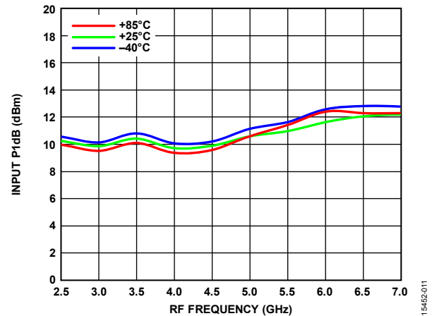
Figure 11. Input P1dB vs. RF Frequency at Various Temperatures
