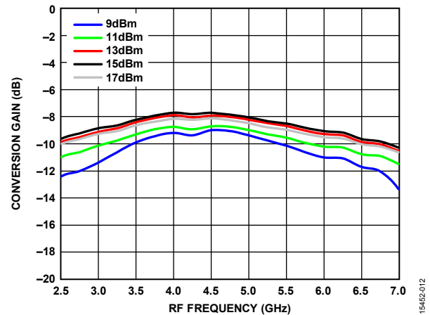
Figure 12. Conversion Gain vs. RF Frequency at Various LO Powers
