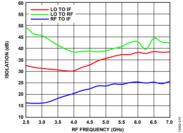
Figure 10. Isolation vs. RF Frequency
