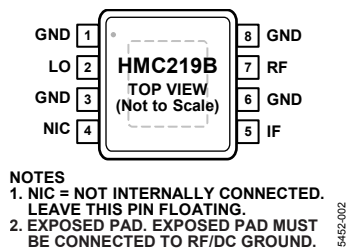
Figure 2. Pin Configuration
