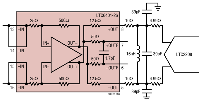
Figure 6. LTC6401-26 with 165MHz Output Bandpass Filter
