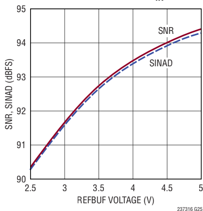
SNR, SINAD vs \text{REFBUF} , f_{\text{IN}} = 1\text{kHz}
