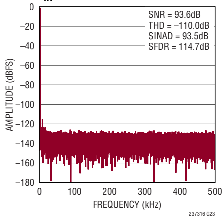
32k Point FFT f_{\text{SAMPL}} = 1\text{Msps} , f_{\text{IN}} = 1\text{kHz}
