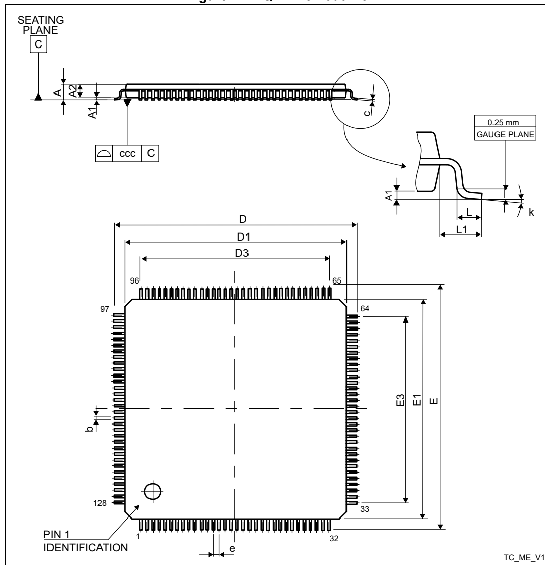
Figure 74. LQFP128 - outline
