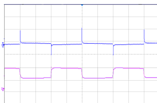
Figure 5 Dynamic response for 25% load step (25% ~ 50% ~ 25%) and 1A/μs slew rate, (2ms/div), see Figure 11 for test configuration; CH1-output voltage (50mV/div); CH2-output current (10A/div)
