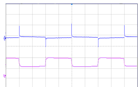
Figure 5 Dynamic response for 25% load step (25% ~ 50% ~ 25%) and 1A/ \mu s slew rate, (2ms/div), see Figure 11 for test configuration; CH1-output voltage (50mV/div); CH2-output current (10A/div)
