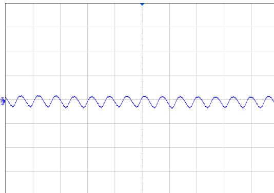
Figure 3 Input reflected ripple current (5 \mu s /div, 10mA/div), see Figure 15 for test configuration
