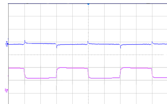
Figure 4 Dynamic response for 25% load step (25% ~ 50% ~ 25%) and 0.1A/ \mu s slew rate, (2ms/div), see Figure 11 for test configuration; CH1-output voltage (50mV/div); CH2-output current (10A/div)
