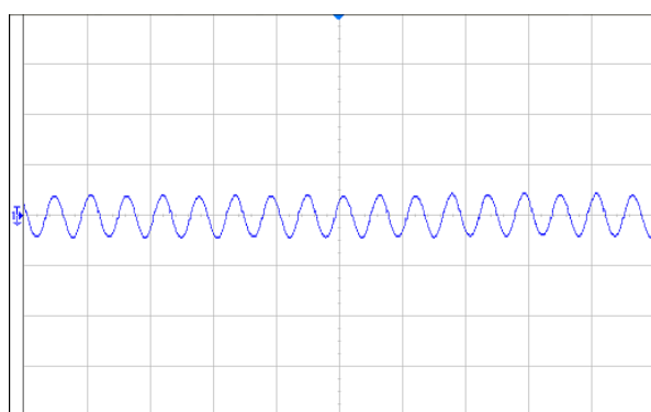
Figure 2 Output ripple & noise (5 \mu s /div, 50mV/div), see Figure 15 for test configuration
